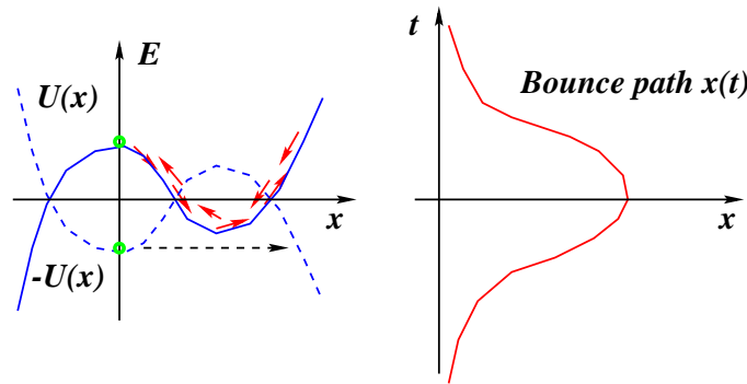
Figure 1: Classical bounce path for tunneling out of a metastable state.
