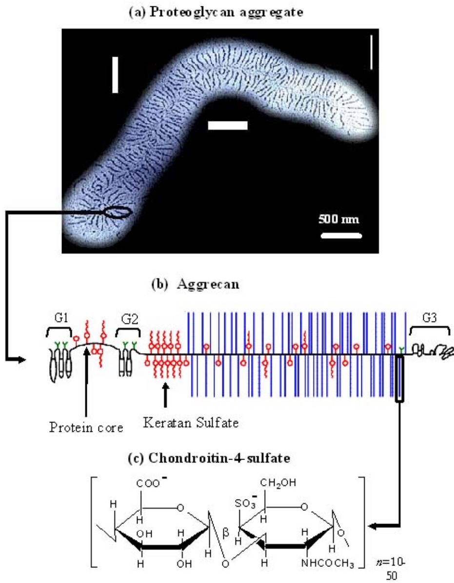
Figure 1. Structural hierarchy of aggrecan in cartilage: (a) electron microscopy of aggrecan and the aggregates it forms with hyaluronan and link protein[Rosenberg, 1982 #627]; (b) aggrecan core protein contains 3 globular domains (G1, G2, G3); the CS-GAG attachment region is composed of a variable keratan sulfate region and 2 chondroitin sulfate regions (CS-1 and CS-2) distinguished by their sequence patterns[Hardingham, 1992 #51].
