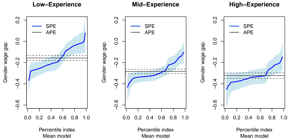
FIGURE 4. APE and SPE of the gender wage gap for women by experience level. Estimates and 90% bootstrap uniform confidence bands based on a linear model with interactions for the conditional expectation function are shown.
