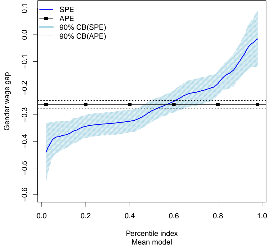
FIGURE 1. The APE and SPE of gender wage gap on the treated female population conditional on job market characters. The estimates are obtained via the plug-in principle and the 90% confidence sets are obtained by empirical bootstrap with 500 repetitions.
