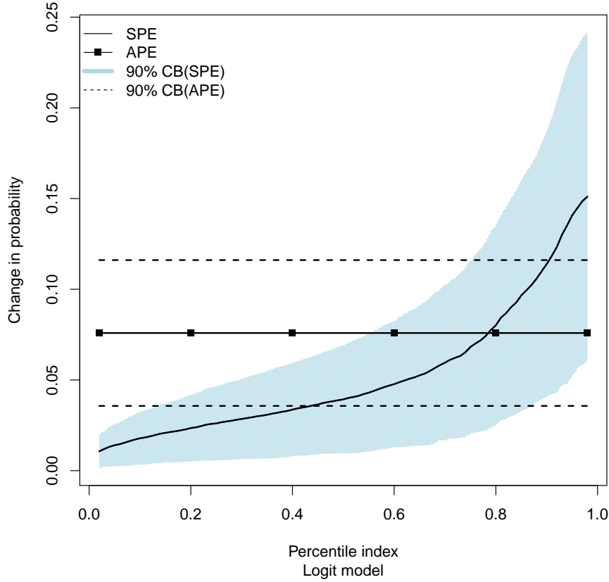
FIGURE 6. The APE and SPE of race on the predicted conditional probabilities for black applicants. 90% confidence sets obtained by empirical bootstrap with 500 repetitions.
