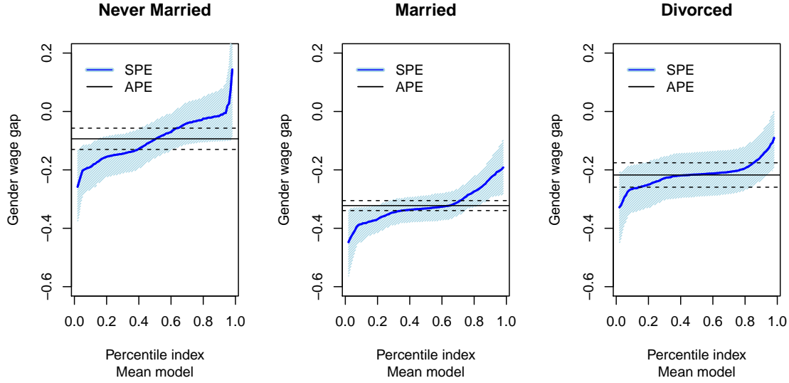
FIGURE 3. APE and SPE of the gender wage gap for women by marital status. Estimates and 90% bootstrap uniform confidence bands based on a linear model with interactions for the conditional expectation function are shown.
