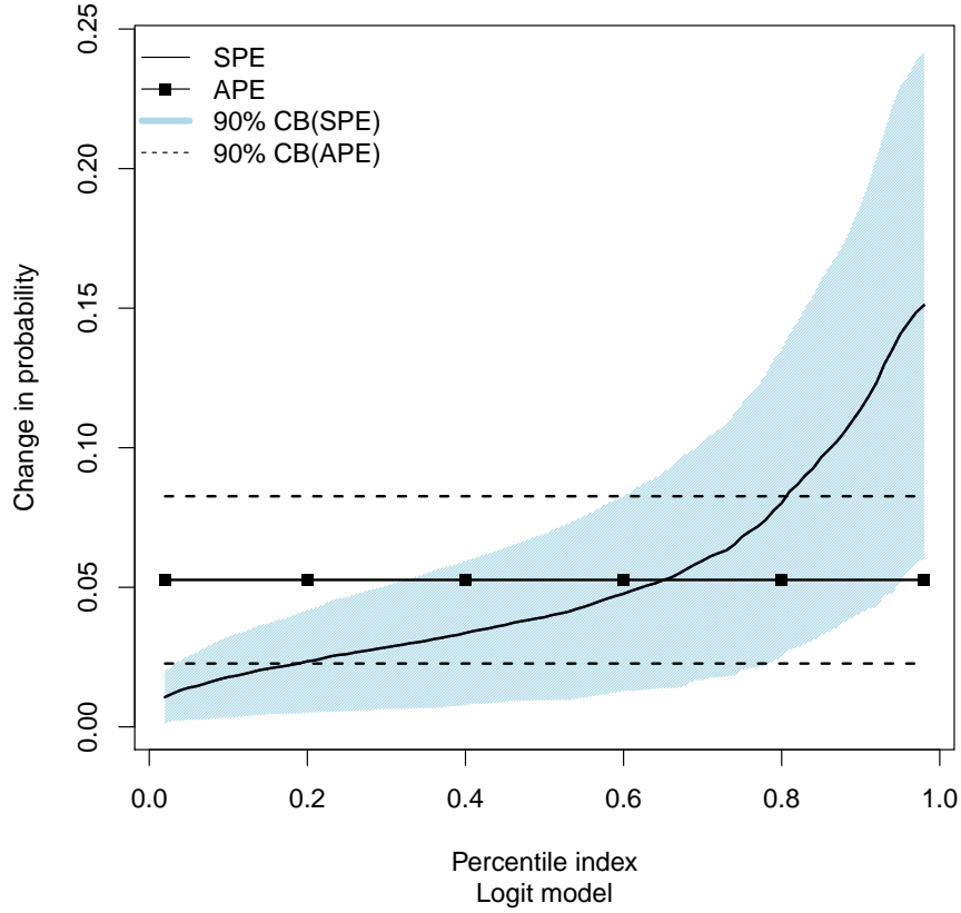
FIGURE 2. The APE and SPE of being black on the probability of mortgage denial conditional on applicant characteristics for the entire population. The estimates are obtained via the plug-in principle and the 90% confidence sets are obtained by empirical bootstrap with 500 repetitions.
