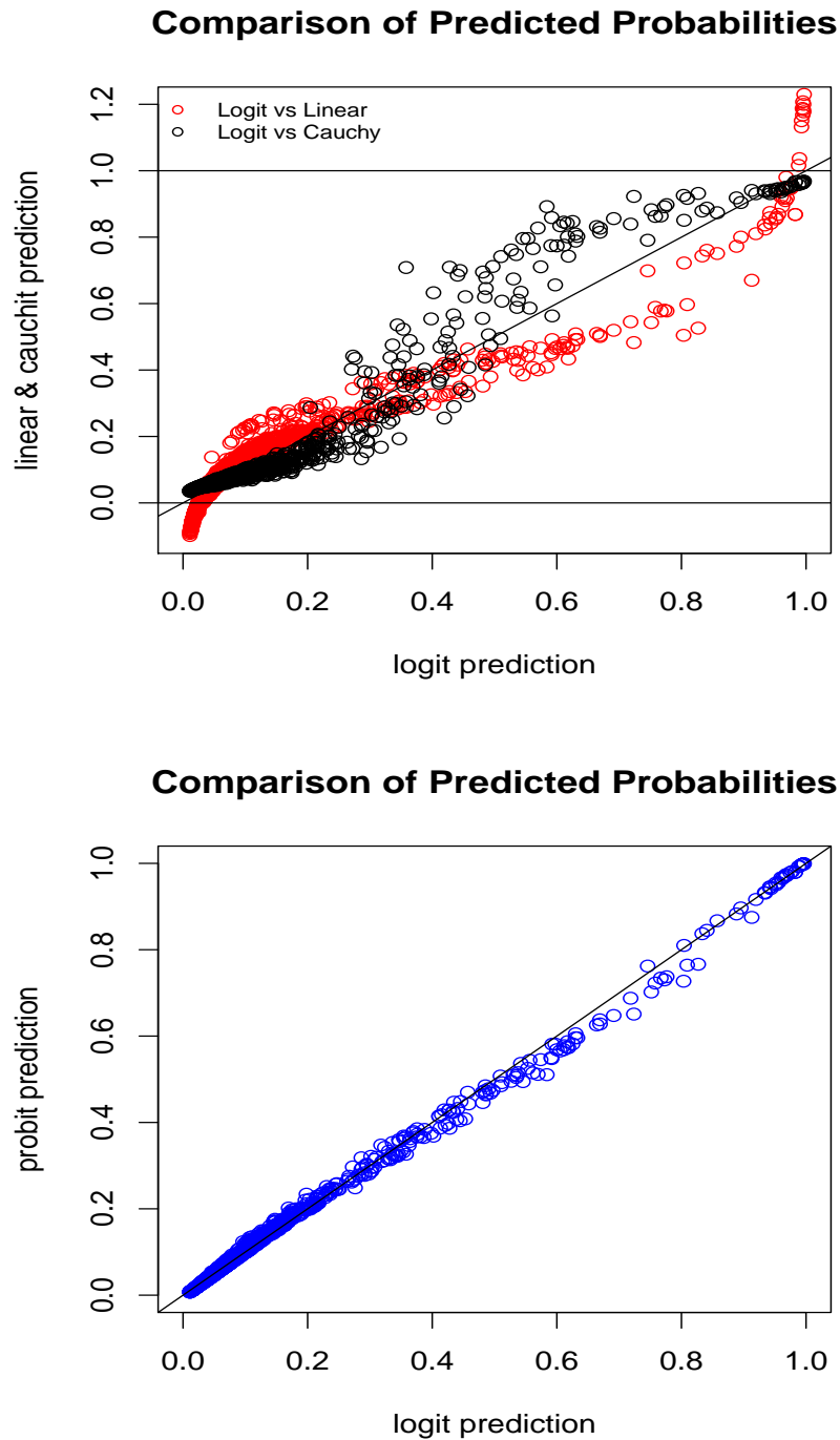
FIGURE 5. Comparison of predicted conditional probabilities of mortgage denial. The top panel compares cauchit and linear against the logit model. The bottom panel compares the probit vs logit models.
